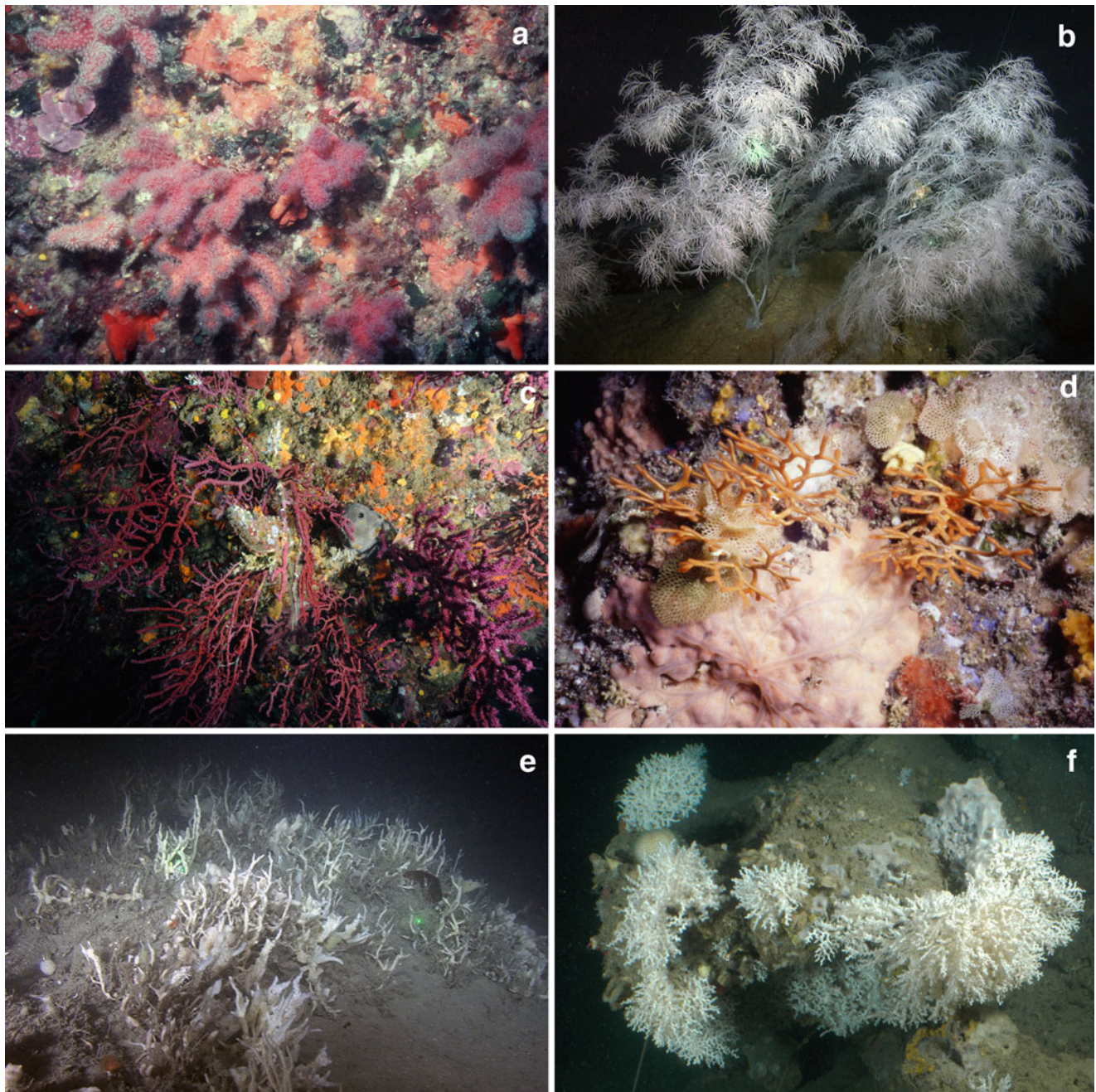
Fig. 12.2 Several examples of rocky bottom communities dominated by sessile organisms in the western Mediterranean: (a) cirralittoral community dominated by the alcyonarian Alcyonium acaule at 20 m depth in the Medes Islands (NW Mediterranean) (foto by J.M. Gili); (b) cirralittoral community dominated by the black coral Antipathella subpinnata at 120 m depth in Son Bou Canyon in Menorca Channel (NW Mediterranean); (c) coralligenous community dominated by the gorgonian Paramuricea clavata at 45 m depth in the Cap de Creus (NW Mediterranean) (Photo by Aldo Ferrucci); (d) cirralittoral community
