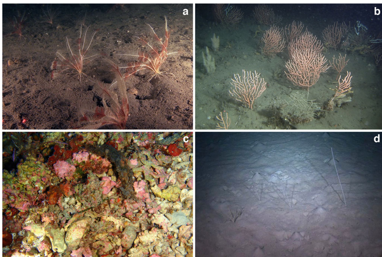
Fig. 12.4 Characteristic assemblages and zoobenthic communities on soft-bottoms: continental shelf detritic communities in the Cap de Creus (NW Mediterranean) at 120 m depth ( a ) facies with Leptometra phalangium at; ( b ) facies dominated by gorgonians Eunicella sp. and sponges (photographs a and b by NEMO-ICM-Gavin Newman);
