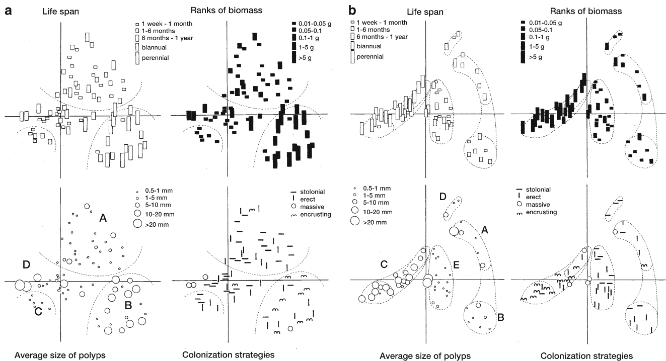
Fig. 12.6 Two examples of ecological strategies present in the different communities from an extensive survey in the Medes Islands (a) and along the Catalan coast (b) (NW Mediterranean). The 104 benthic cnidarian species considered have been ordered by means of a Principal Component Analysis (Figure modified from Gili et al. 1989, see this paper for more information and species list). (a) A mediolittoral community and assemblages of photophilic algae; B circalittoral community mainly
