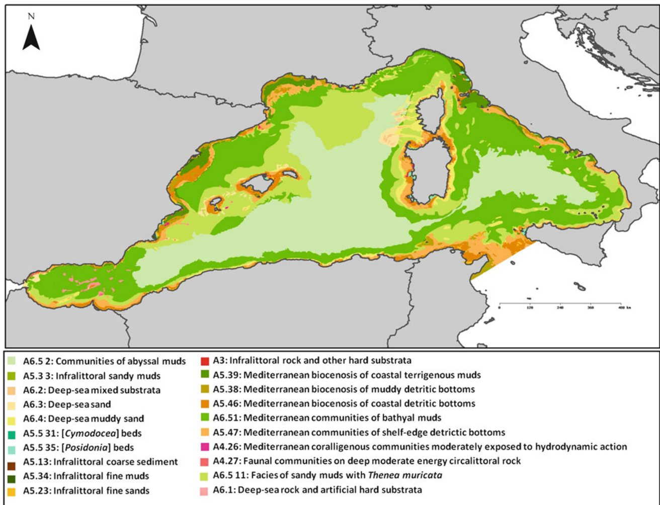
Fig. 12.5 Benthic cartography (EUSaMap) from the Northwestern Mediterranean following EUNIS classification (Adapted from http://jncc.defra.gov.uk/page-5020 )
